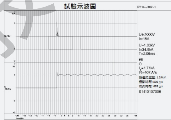
1000V In15A/34.9kA
